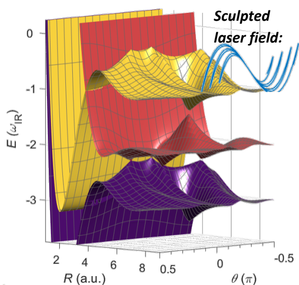
Light-induced potentials of the molecular hydrogen cation ( H_2^+ ) in a
